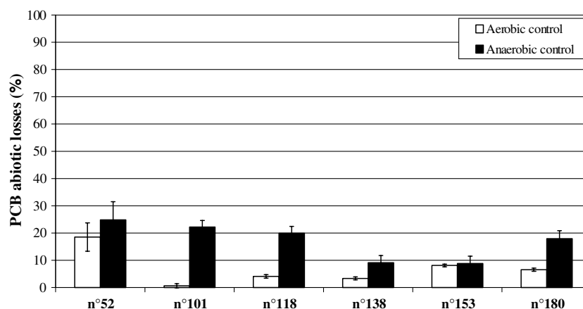
Figure 1. Abiotic losses of six priority PCBs in anaerobic and aerobic control sludge reactors at steady state.
