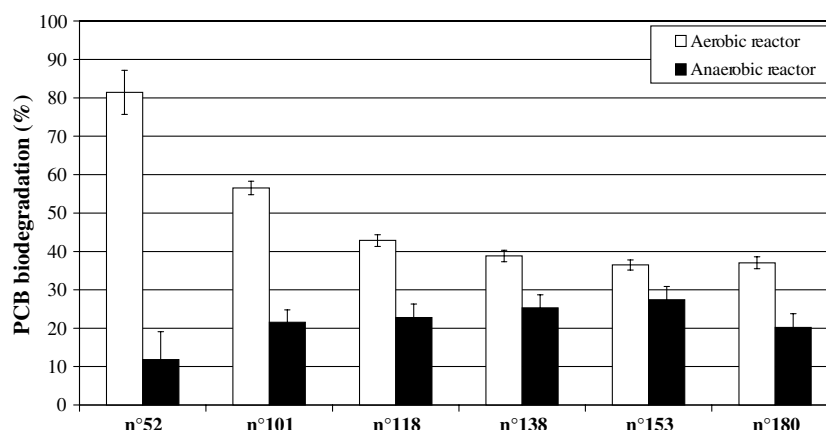
Figure 3. Actual PCB biodegradation after correction by the abiotic losses in anaerobic and aerobic biological reactors at steady state.
