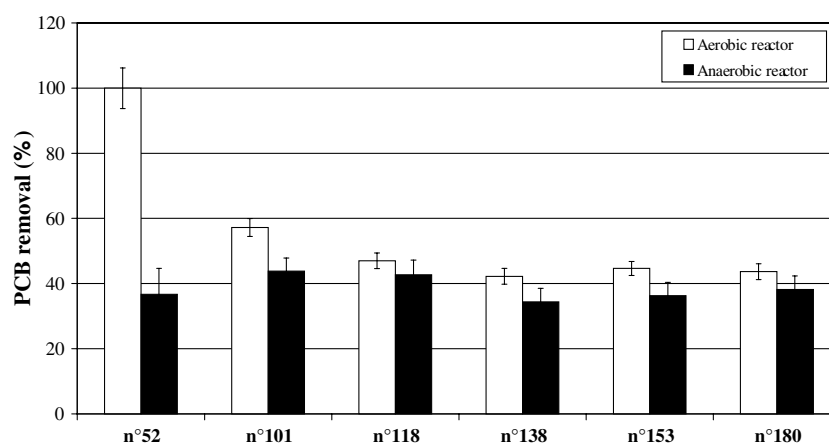
Figure 2. PCB removal in anaerobic and aerobic biological reactors at steady state.
